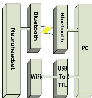
Figure 4. System architecture, transmitter block.
