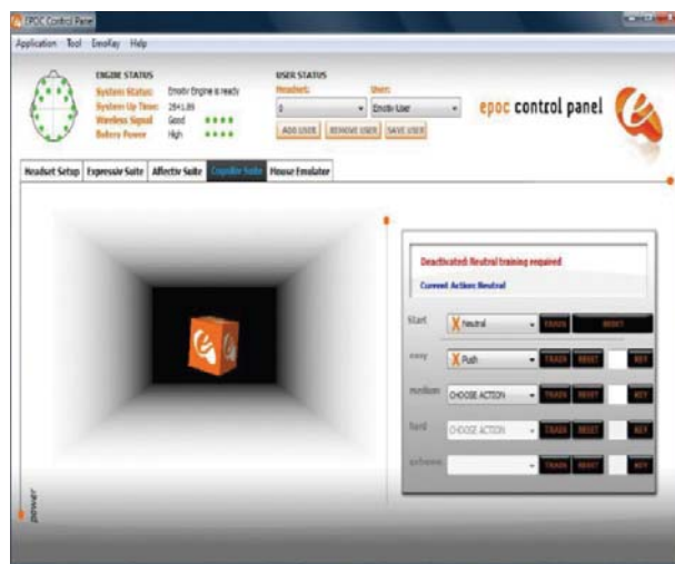
Figure 7. Cognitive Suite.
