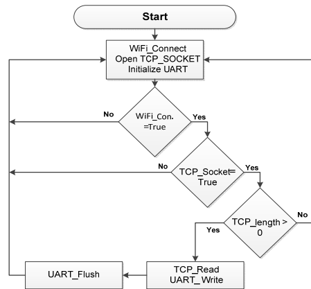
Figure 12. Client action while receiving subject's thought.
