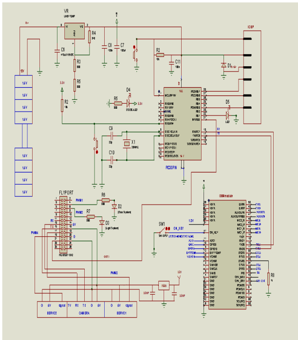
Figure 9. Circuit diagram of the receiver side.
