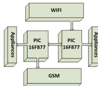
Figure.5 System architecture, receiver block.
