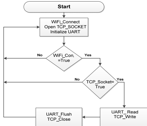
Figure 11. Server action while sending subject's thought.
