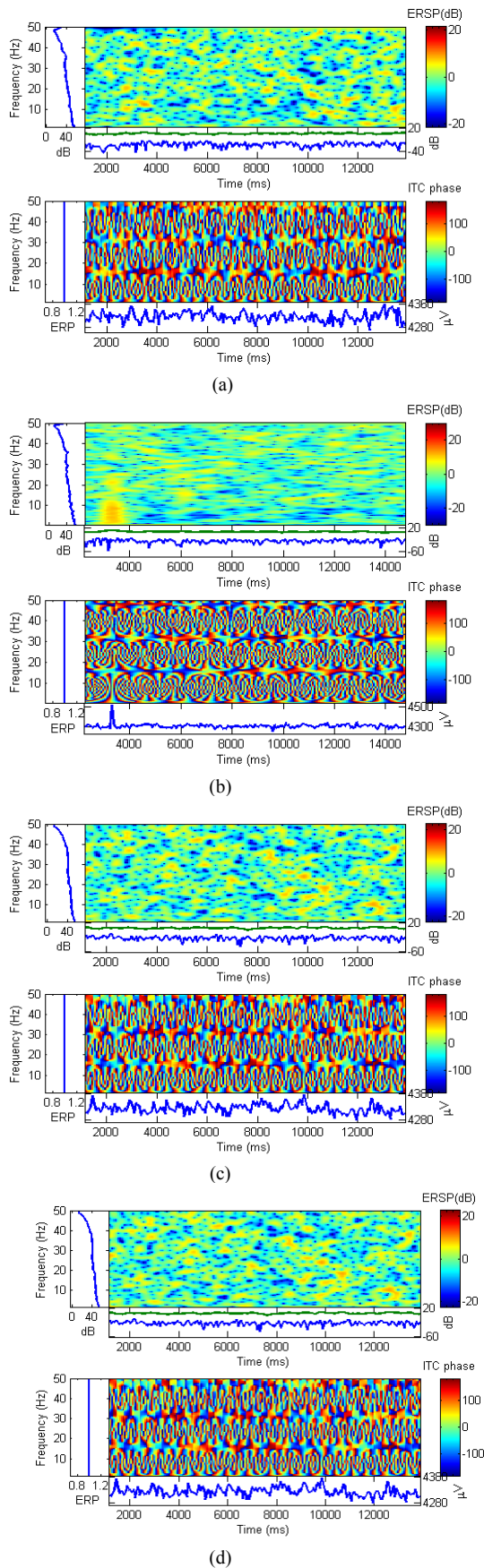
Figure 15. Real-time EEG Measurements in TestBench: (a) Left, (b) Right, (c) Pull, (d) Push. The data shown are processed using EEGLAB
