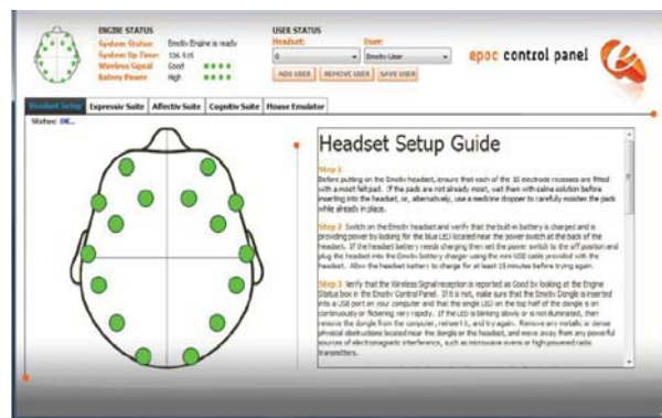
Figure 6. Control Panel.
