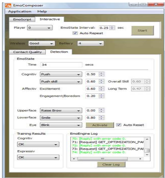
Figure 13. EmoComposer suite.
